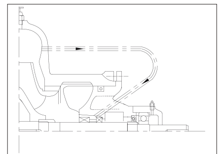
DETAILS AT - A
